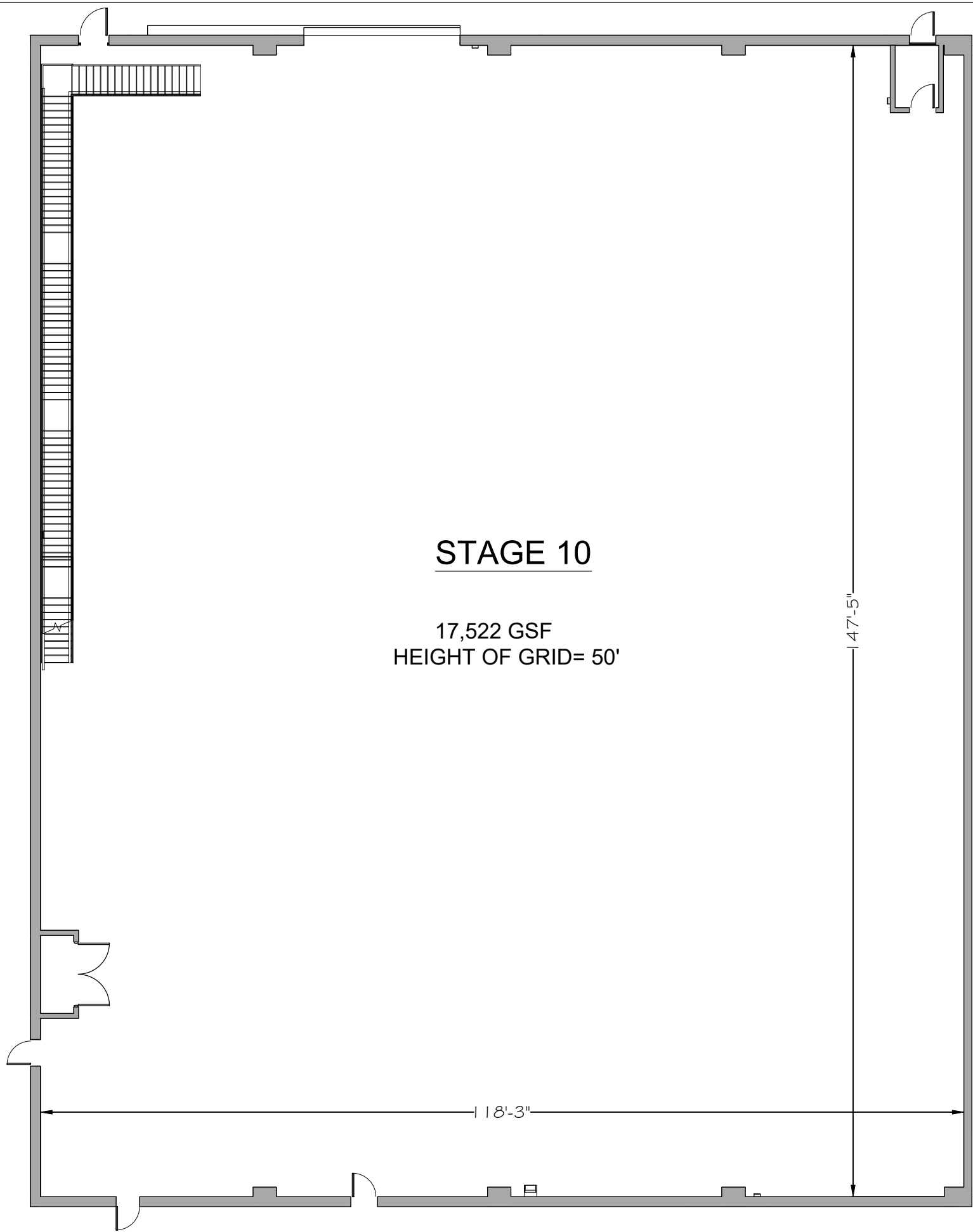
STAGE FLOOR PLAN
