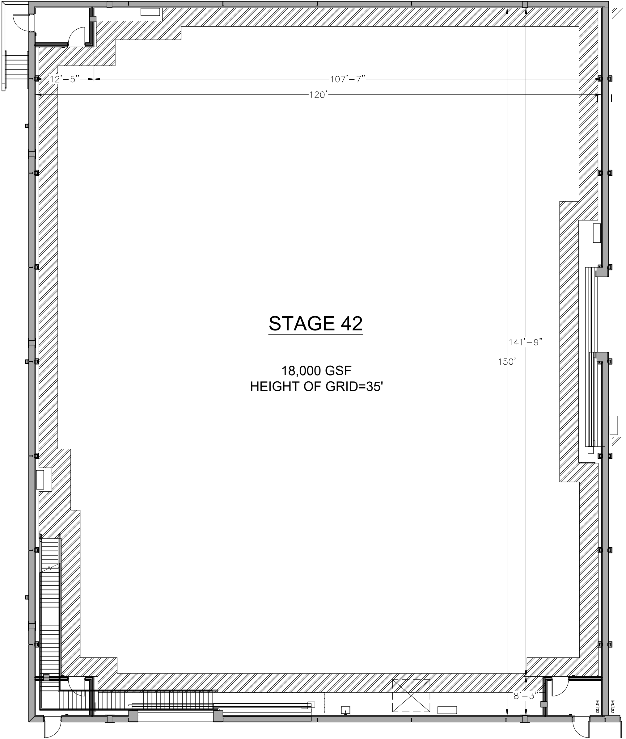
STAGE FLOOR PLAN
